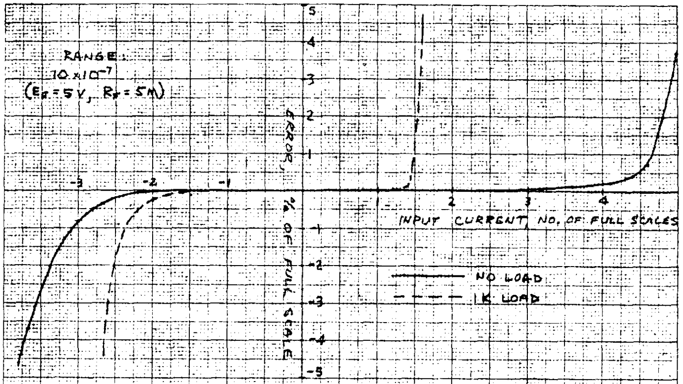
MODEL 410 OVERLOAD CHARACTERISTICS FIG. 1
